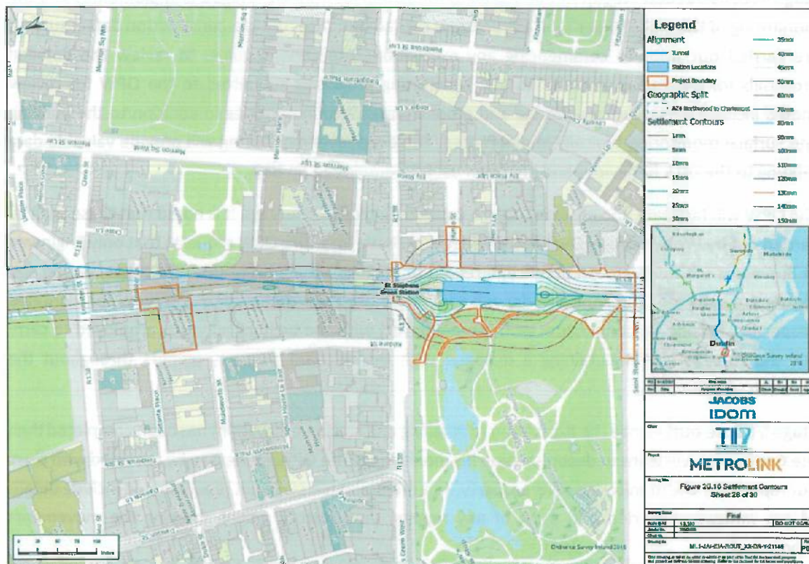
Figure 17. Settlement Contours (Extract from ML1-JAI-EIA-ROUT_XX-DR-Y-21148)
